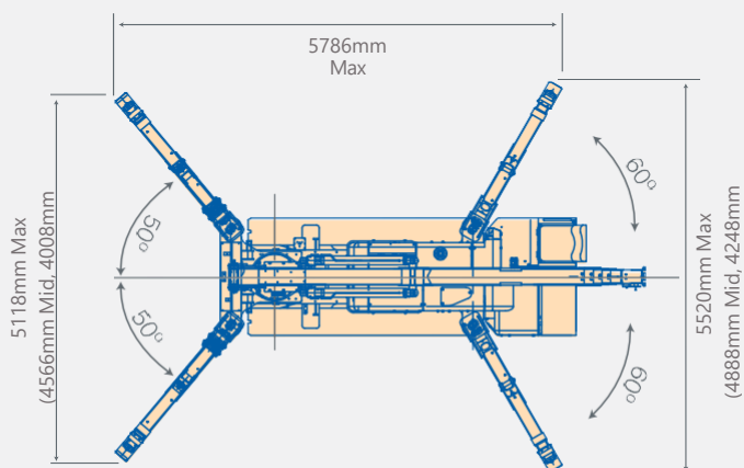
Diagram shows outriggers at maximum position
