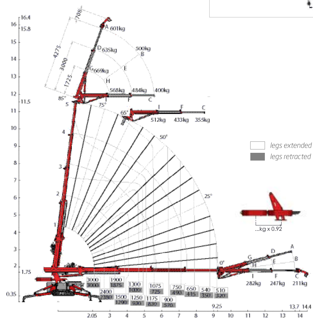
With counterweight
